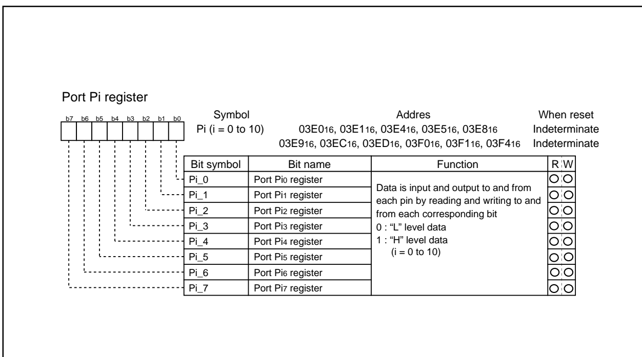
Figure 118. Port register
