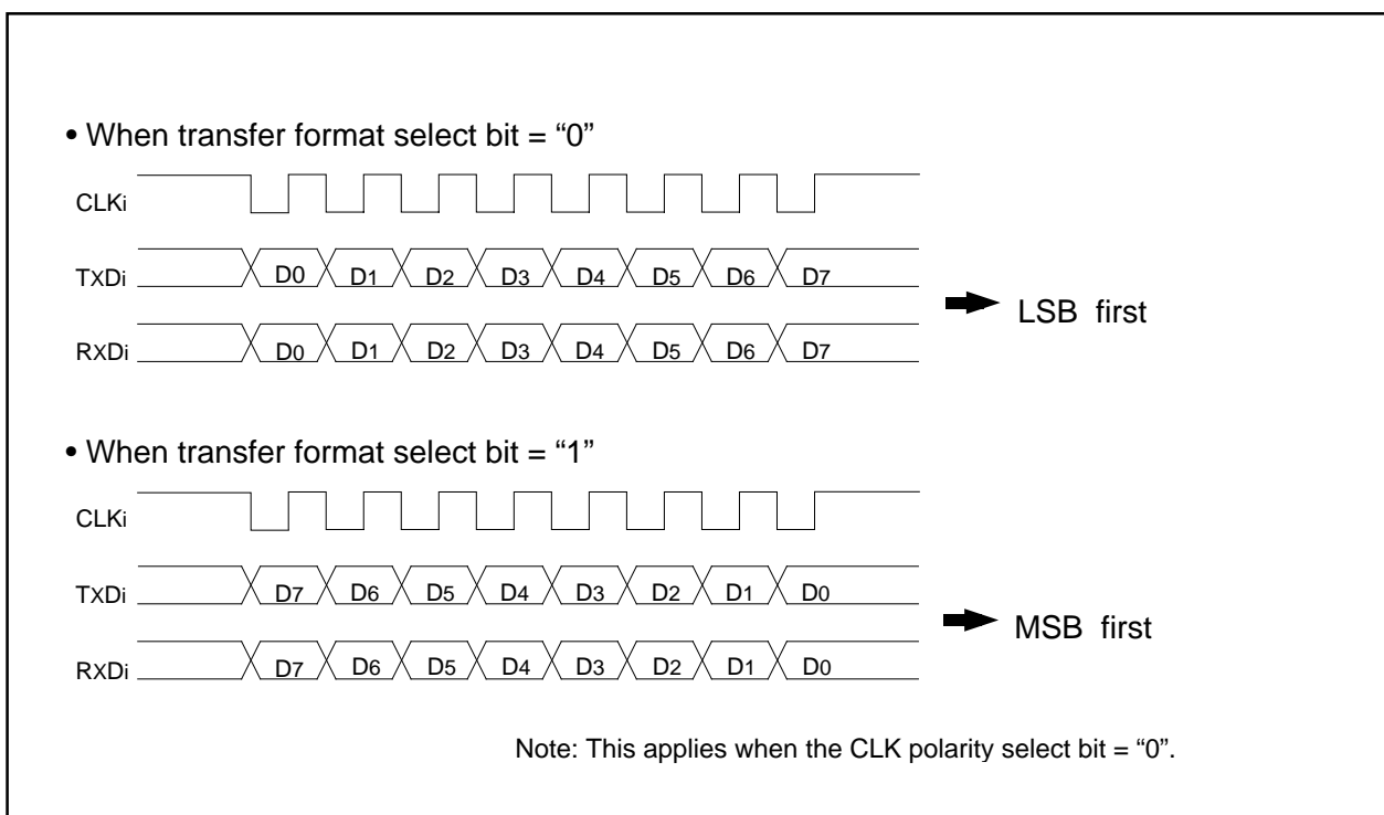
Figure 82. Transfer format
