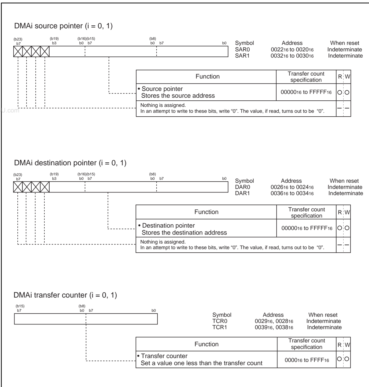
Figure 2.10.3. DMAC-related registers (2)
