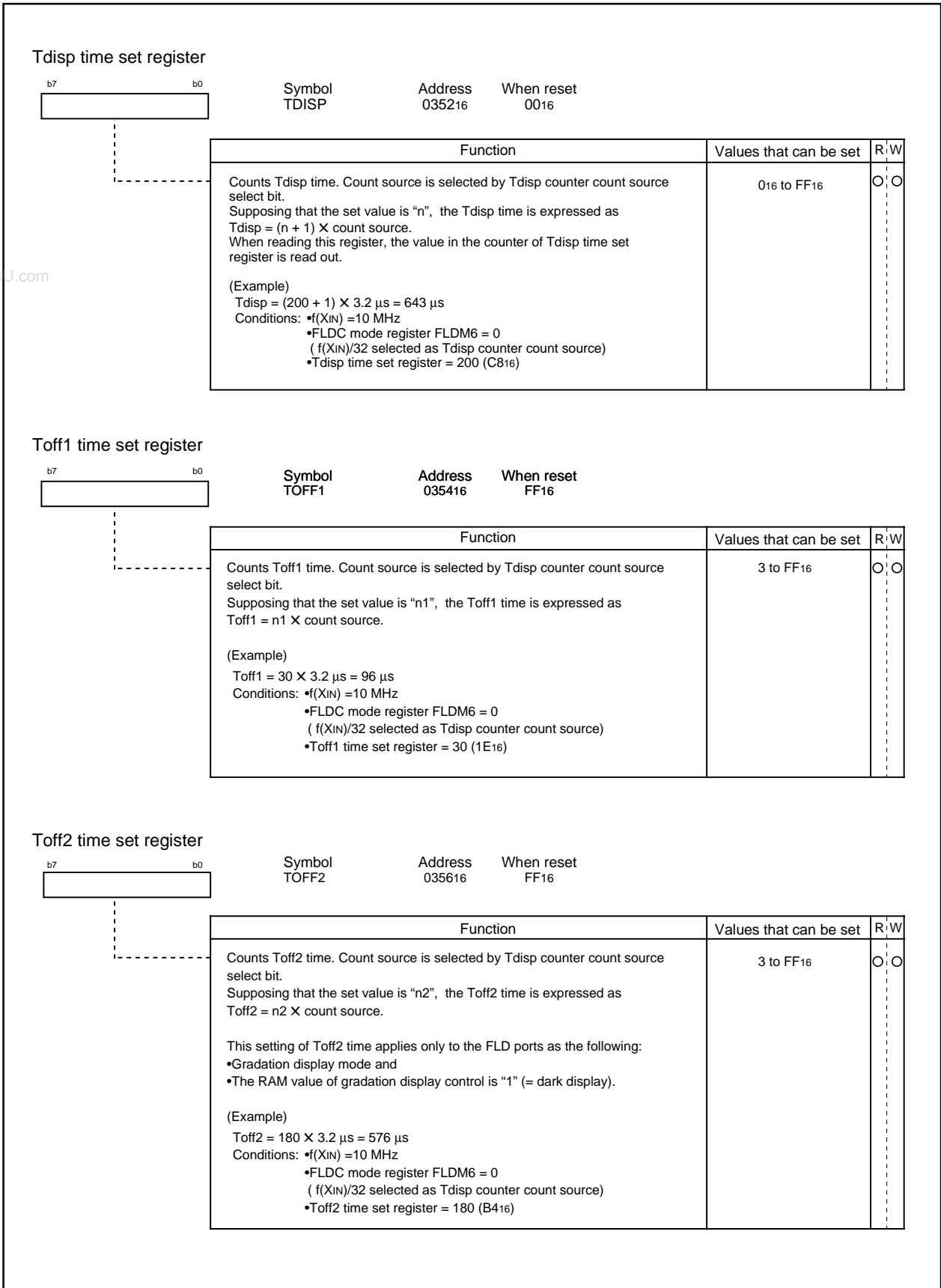
Figure 2.7.3. FLDC related-registers (2)
