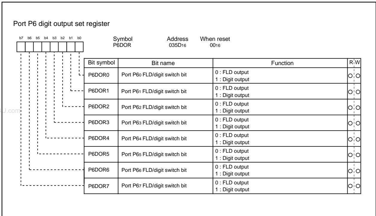
Figure 2.7.6. FLDC related-registers (5)
