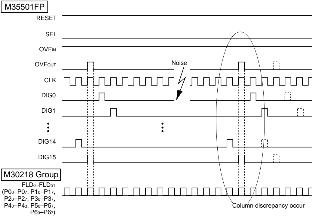
Figure 2.7.23. Operation timing of FLD automatic display
