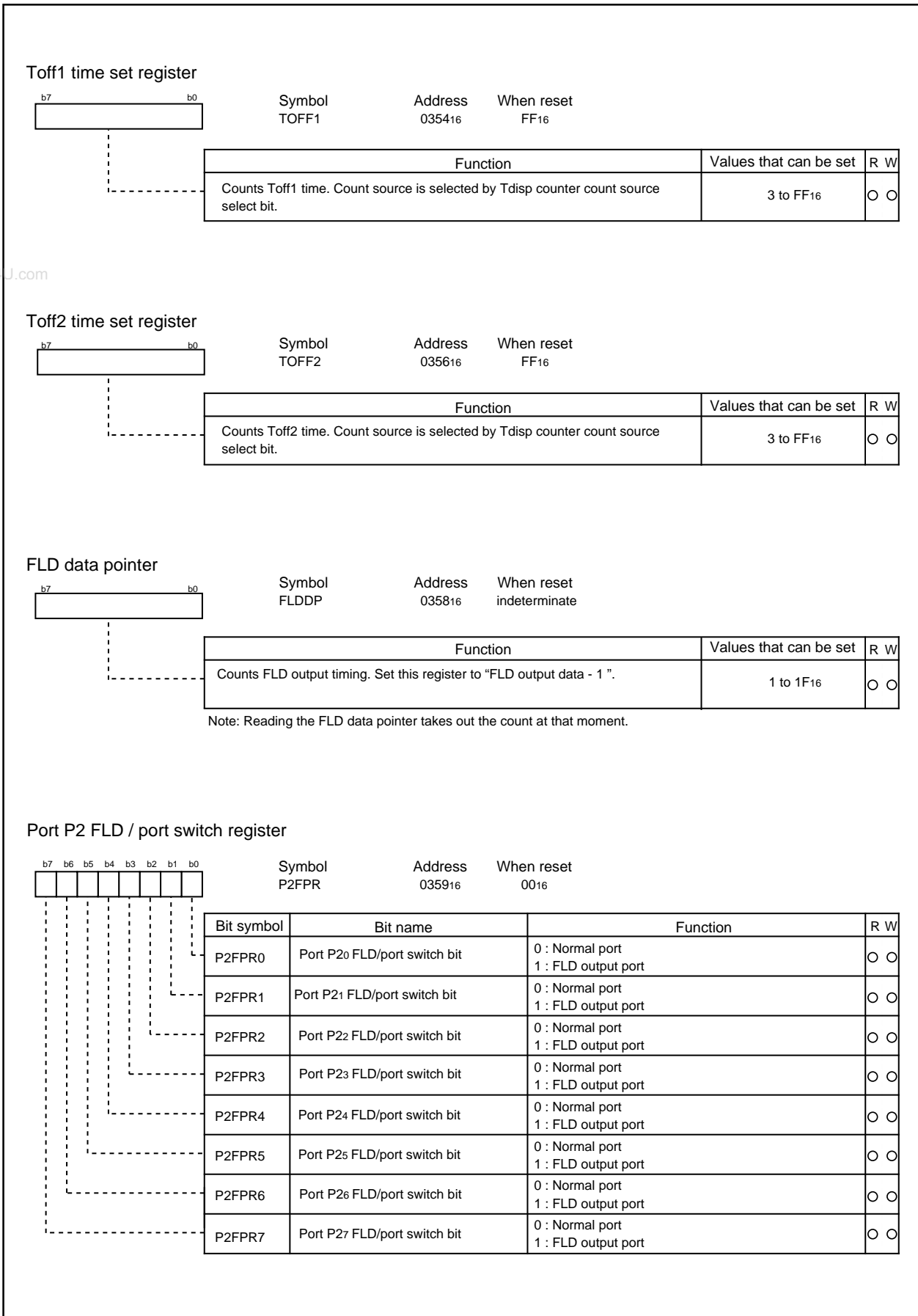
Figure 40. FLDC-related Register(2)
