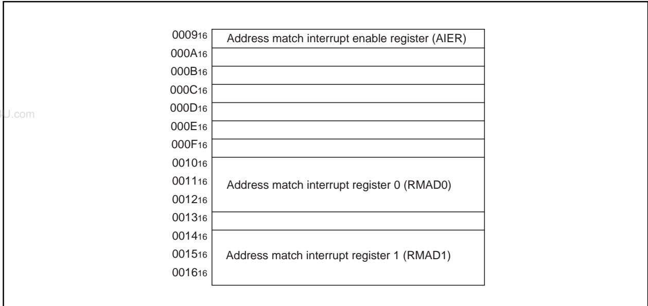
Figure 2.13.2. Memory map of address match interrupt-related registers
