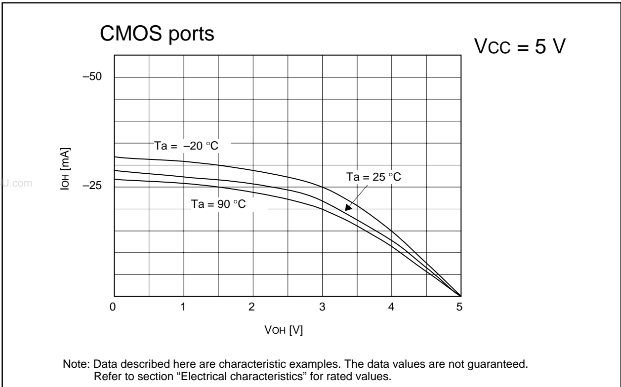
Figure 5.1.1. I_{OH} - V_{OH} standard characteristics of ports P44 to P47, P7 to P10 ( V_{CC} = 5V )
