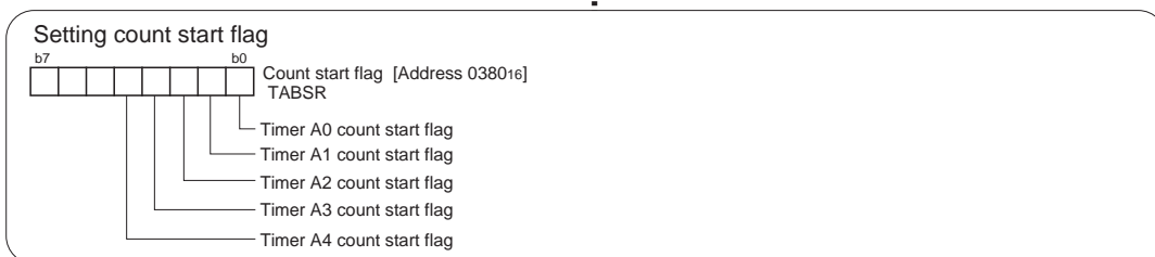
Figure 2.2.13. Set-up procedure of event counter mode, reload type selected
