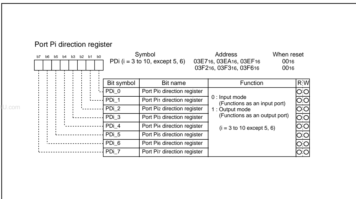
Figure 117. Direction register
