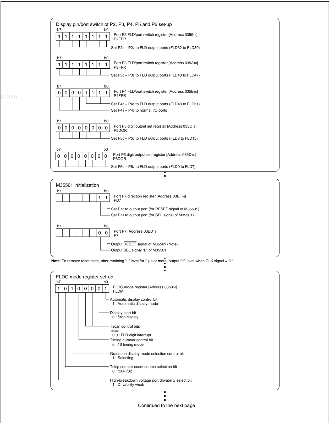
Figure 2.7.20. Set-up procedure for FLD automatic display (1)
