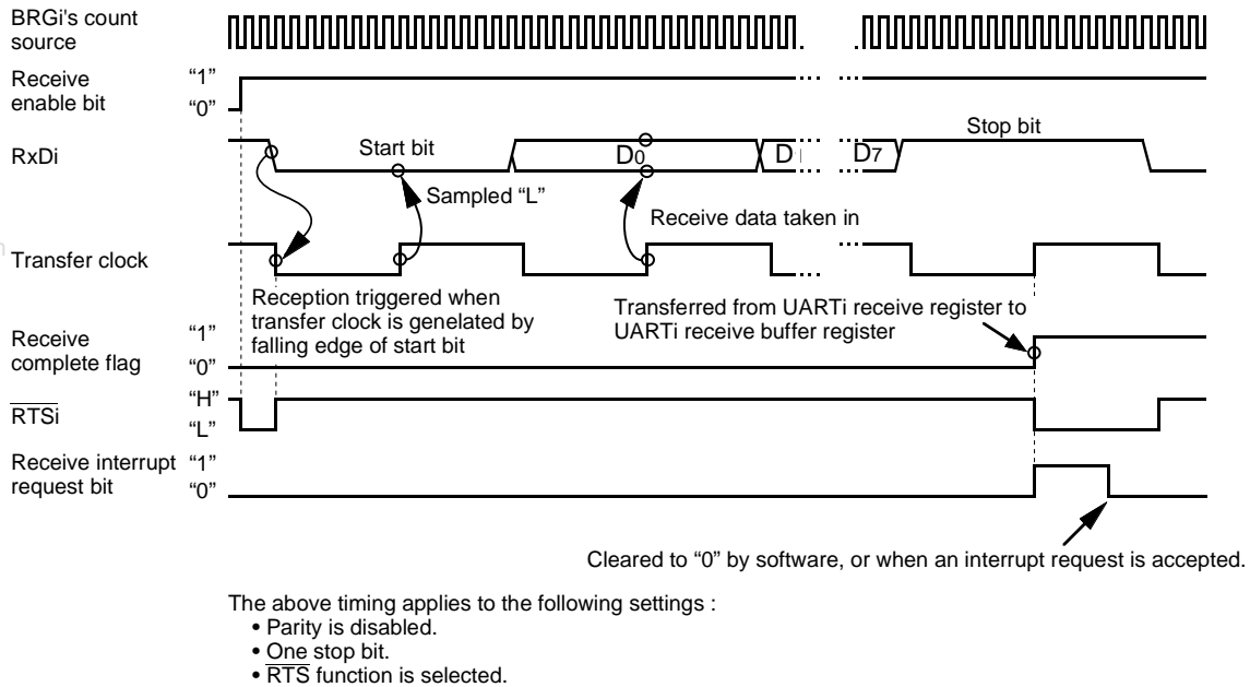
Figure 86. Typical receive timing in UART mode
