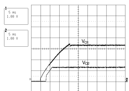
Start up (typ)
