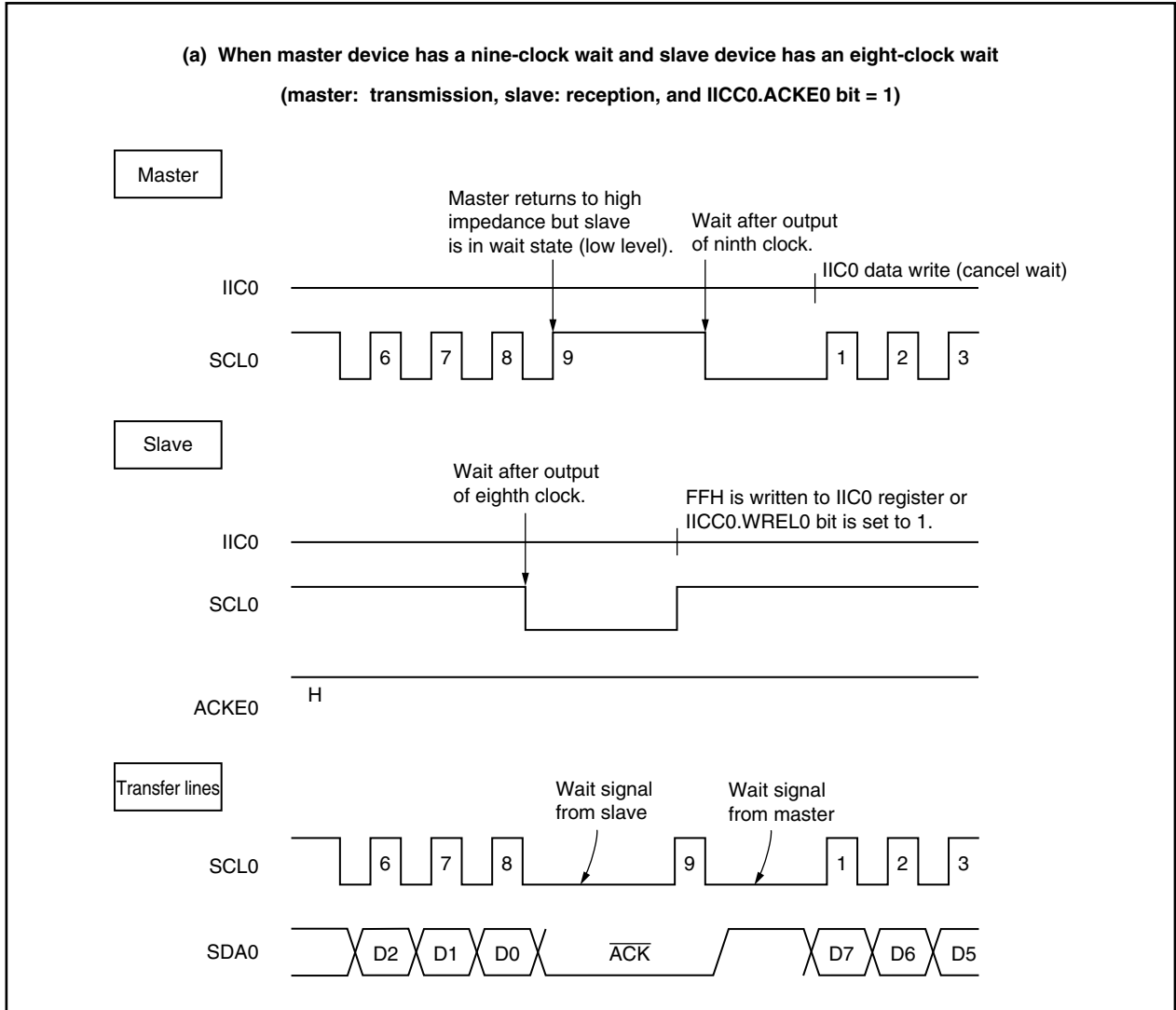
Figure 19-10. Wait Signal (1/2)
