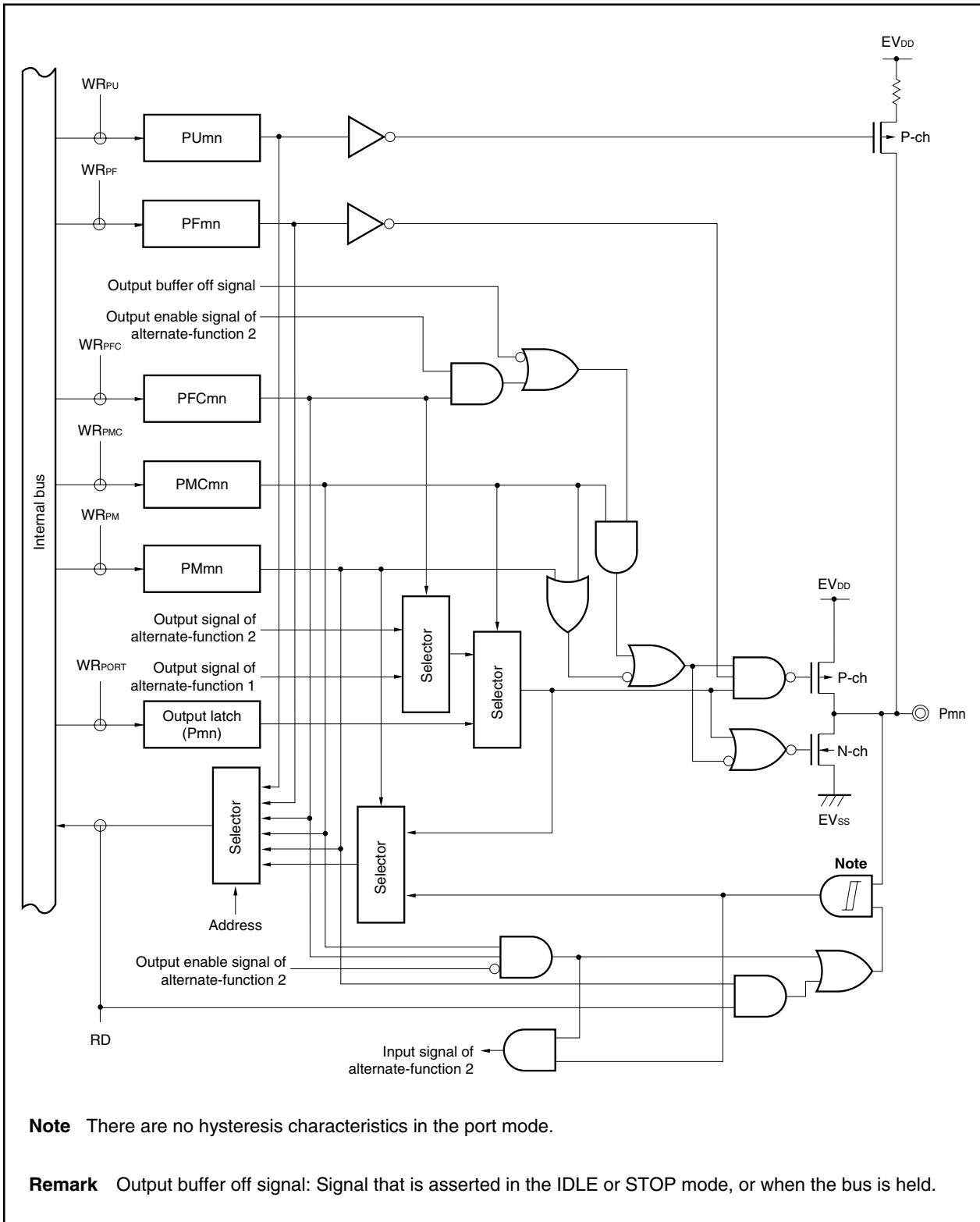
Figure 4-21. Block Diagram of Type G-3
