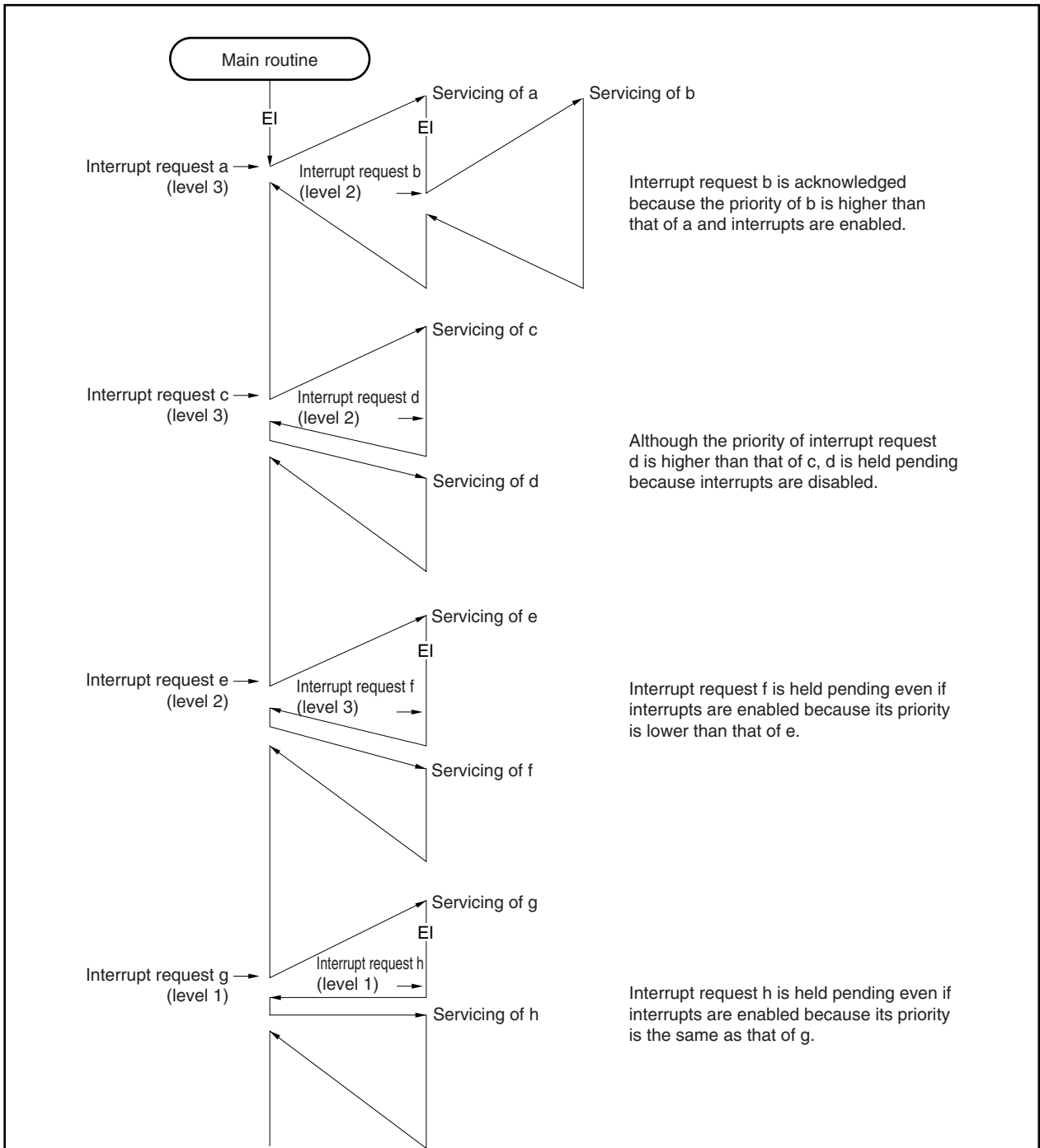
Figure 20-6. Example of Interrupt Nesting (1/2)
