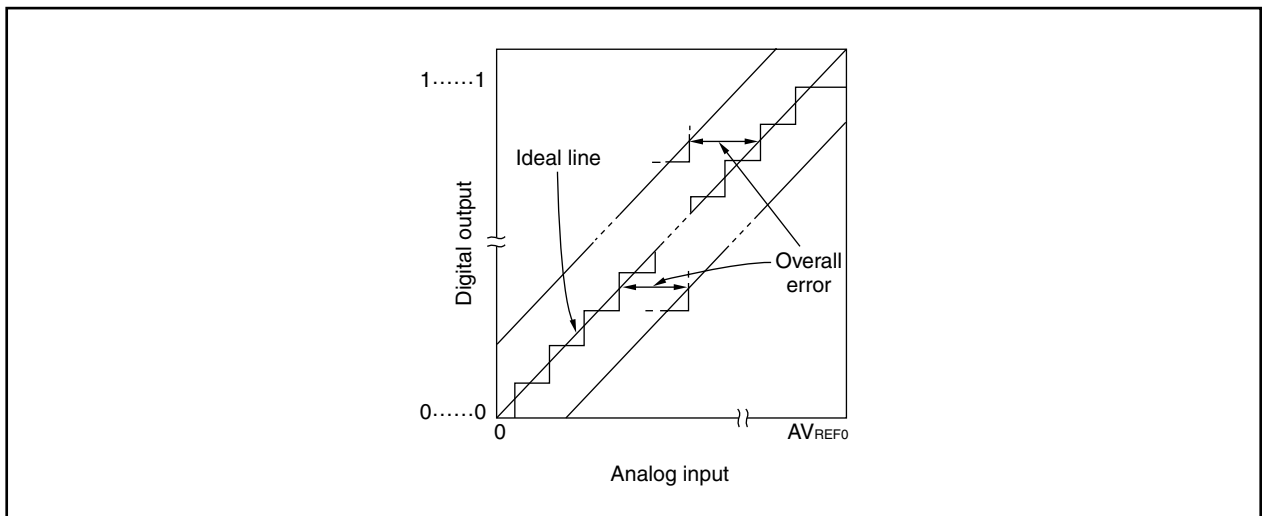
Figure 14-10. Overall Error
