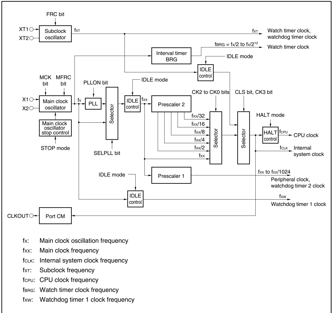
Figure 6-1. Clock Generator
