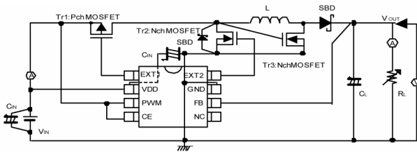
Circuit ③
