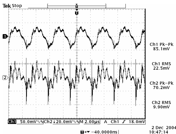
Ripple and noise at full load, 75 V input, ch1 (+)12 V/5 A output, (-)12 V/1.5 A
