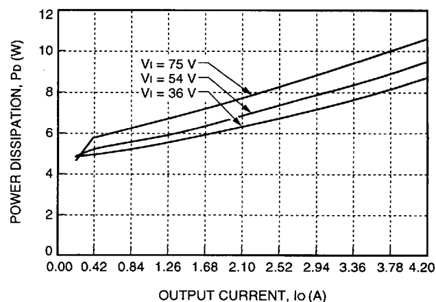
Figure 28. JW050B Power Dissipation vs. Output Current
