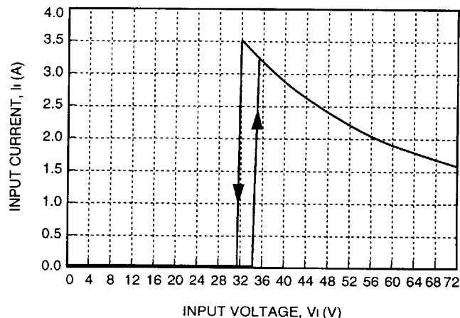
Figure 3. Typical JW100B Input Characteristics at Room Temperature, I_o = 8.3 A
