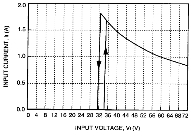
Figure 1. Typical JW050B Input Characteristics at Room Temperature, I_o = 4.2 A
