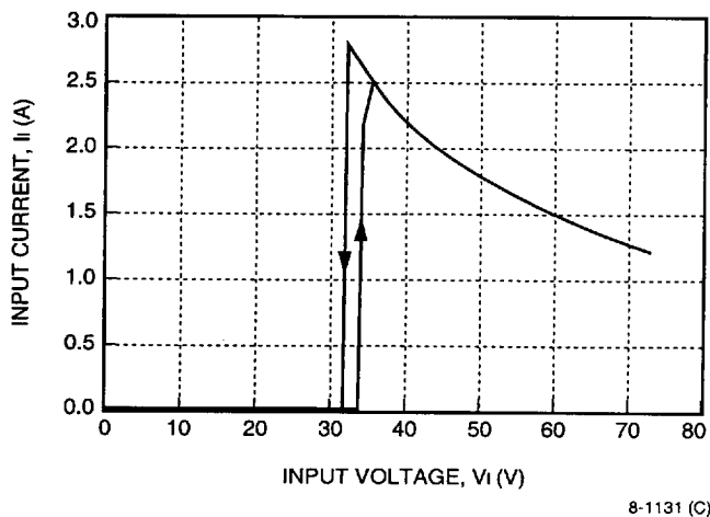
Figure 2. Typical JW075B Input Characteristics at Room Temperature, I_o = 6.3 A
