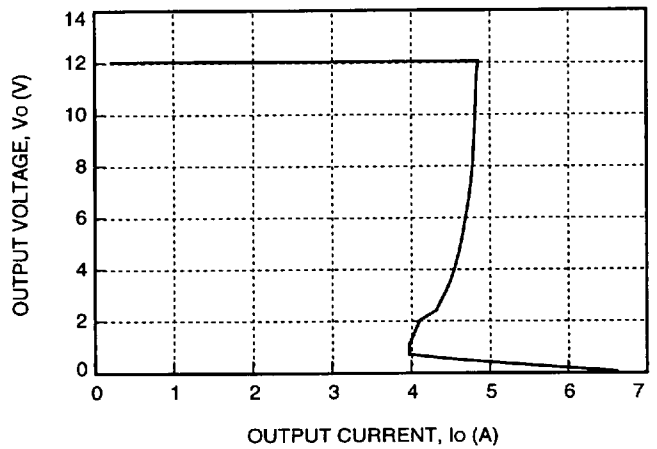
Figure 5. Typical JW050B Output Characteristics at Room Temperature, V_{IN} = 48\text{ V}
