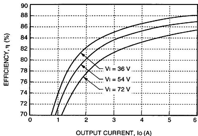
Figure 10. Typical JW075B Converter Efficiency vs. Output Current at Room Temperature
