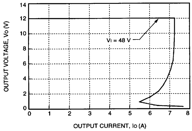
Figure 6. Typical JW075B Output Characteristics at Room Temperature, V_{IN} = 48\text{ V}
