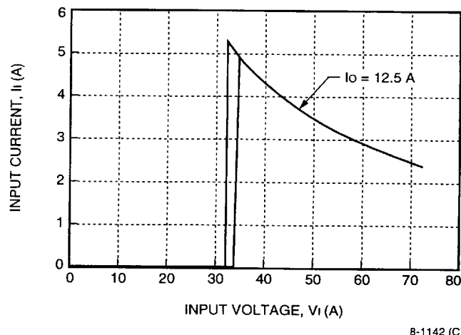
Figure 4. Typical JW150B Input Characteristics at Room Temperature, I_o = 12.5 A
