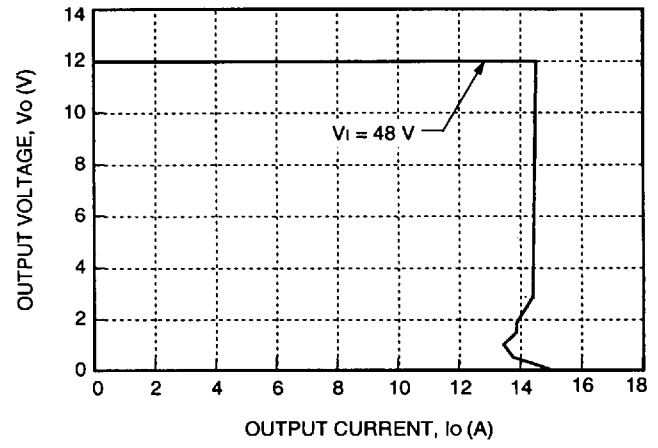
Figure 8. Typical JW150B Output Characteristics at Room Temperature, V_{IN} = 48\text{ V}
