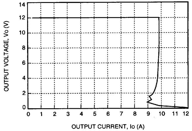
Figure 7. Typical JW100B Output Characteristics at Room Temperature, V_{IN} = 48\text{ V}
