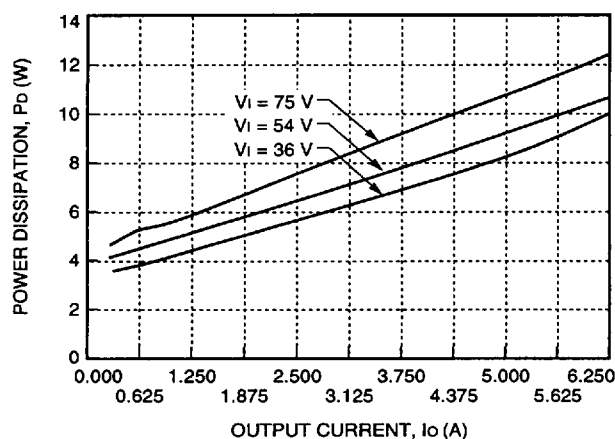
Figure 29. JW075B Power Dissipation vs. Output Current
