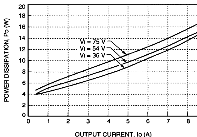
Figure 30. JW100B Power Dissipation vs. Output Current
