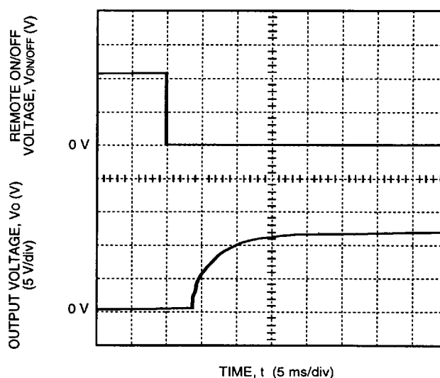
Figure 16. Typical Start-Up from Remote On/Off JW150B1; I_o = Full Load
