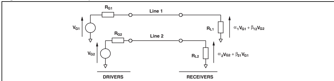
Figure 22. Crosstalk phenomena
