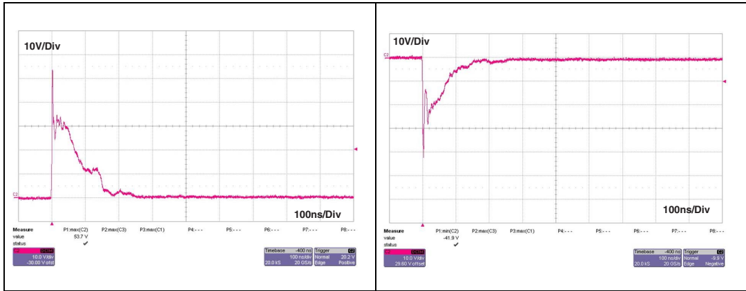
Figure 20. Remaining voltage after the HDMIULC6-2P6 during positive ESD surge
