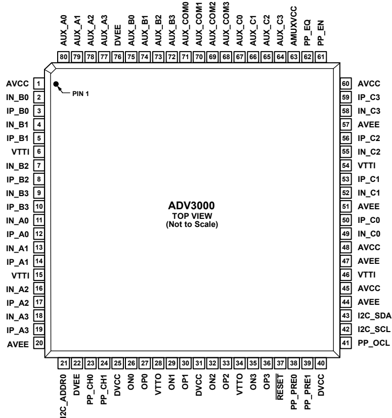
Figure 3. Pin Configuration
