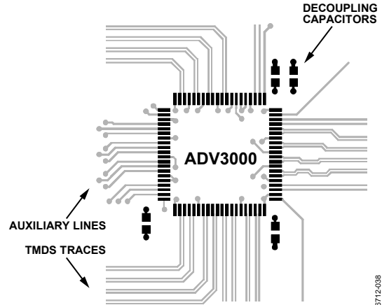
Figure 35. Example Placement of Power Supply Decoupling Capacitors Around the ADV3000
