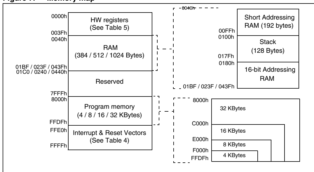
Figure 7. Memory map
