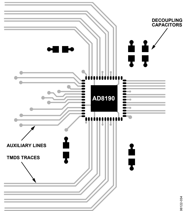
Figure 35. Example Placement of Power Supply Decoupling Capacitors Around the AD8190
