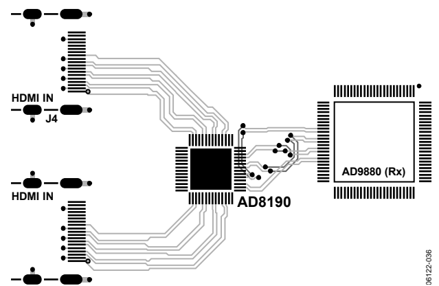
Figure 32. Layout of the TMDS Traces for the AD8190 in an HDMI Standard Revision 1.2a Receive-Compliant Reference Design
