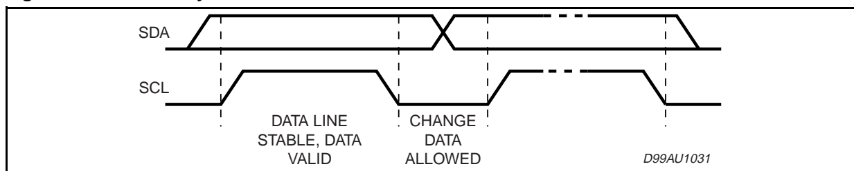
Figure 16: Data Validity on the I 2 C BUS
