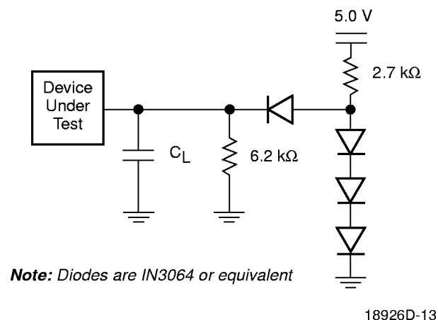
Figure 8. Test Setup
