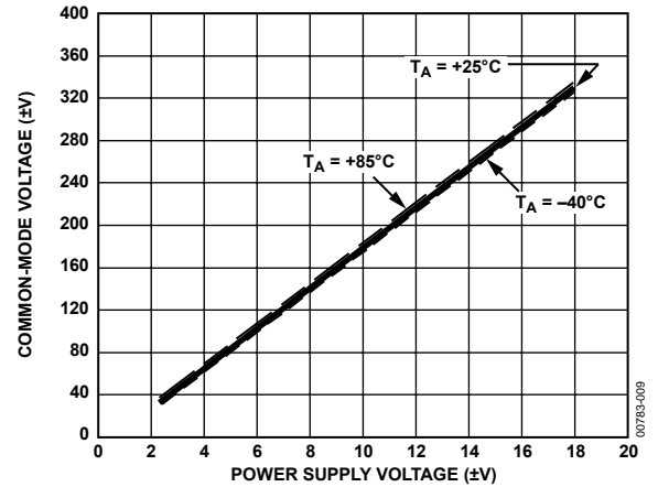
Figure 8. Common-Mode Operating Range vs. Power Supply Voltage
