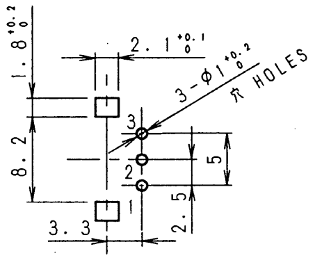
端子取付穴寸法図 (挿入側より見た図) (許容差±0.1) MOUNTING HOLE DETAIL (TOLERANCE±0.1) VIEWED FROM MOUNTING SIDE 板厚 t=1.6
