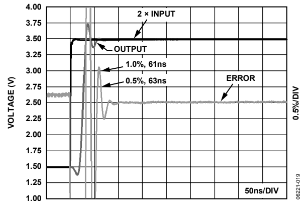
Figure 19. Settling Time
