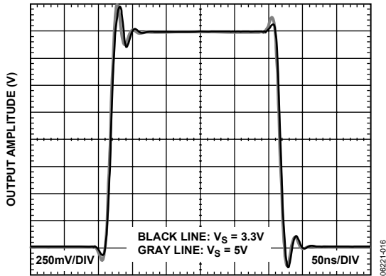
Figure 16. Transient Response
