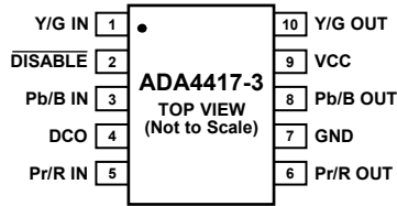
Figure 3. Pin Configuration
