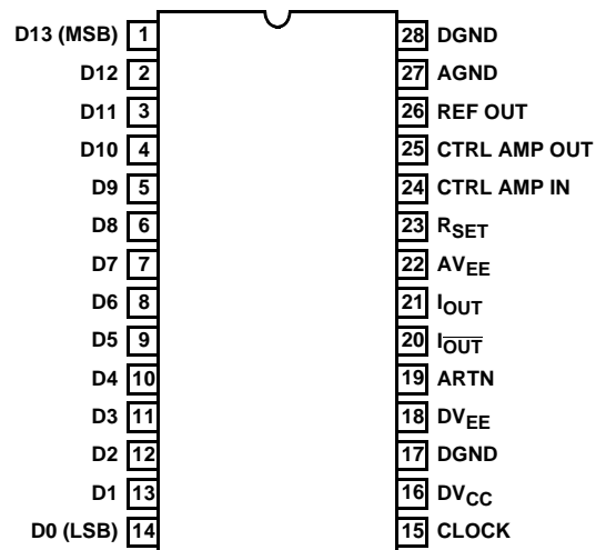
HI5741 (SOIC) TOP VIEW
