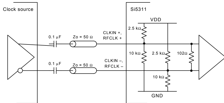
Figure 10. Input Termination for CLKIN and REFCLK (AC Coupled)
