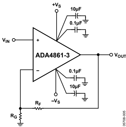
Figure 46. Noninverting Gain
