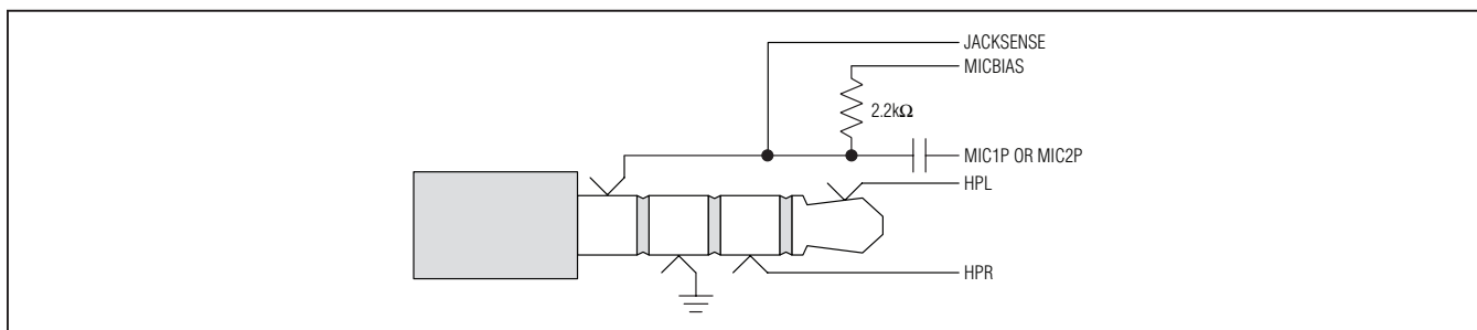
Figure 33. Typical Configuration for Jack Detection
