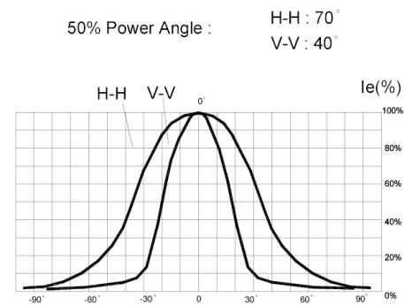
FIG.6 FAR FIELD PATTERN
