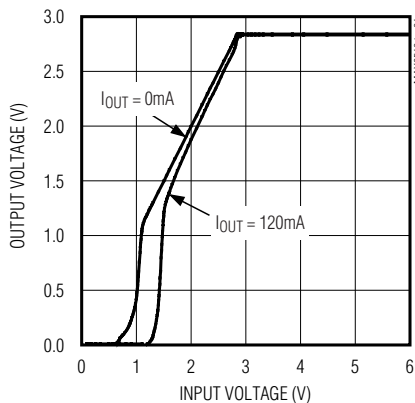
MAX8510 OUTPUT VOLTAGE vs. INPUT VOLTAGE
