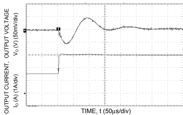
Figure 12. Transient Response to Dynamic Load Change from 50% to 100% of full load (V o = 3.3Vdc, C ext = 2x150 μF Polymer Capacitors).
