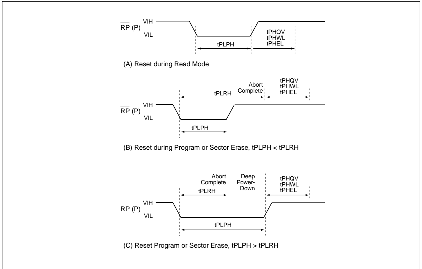
Figure 5. RESET WAVEFORM
