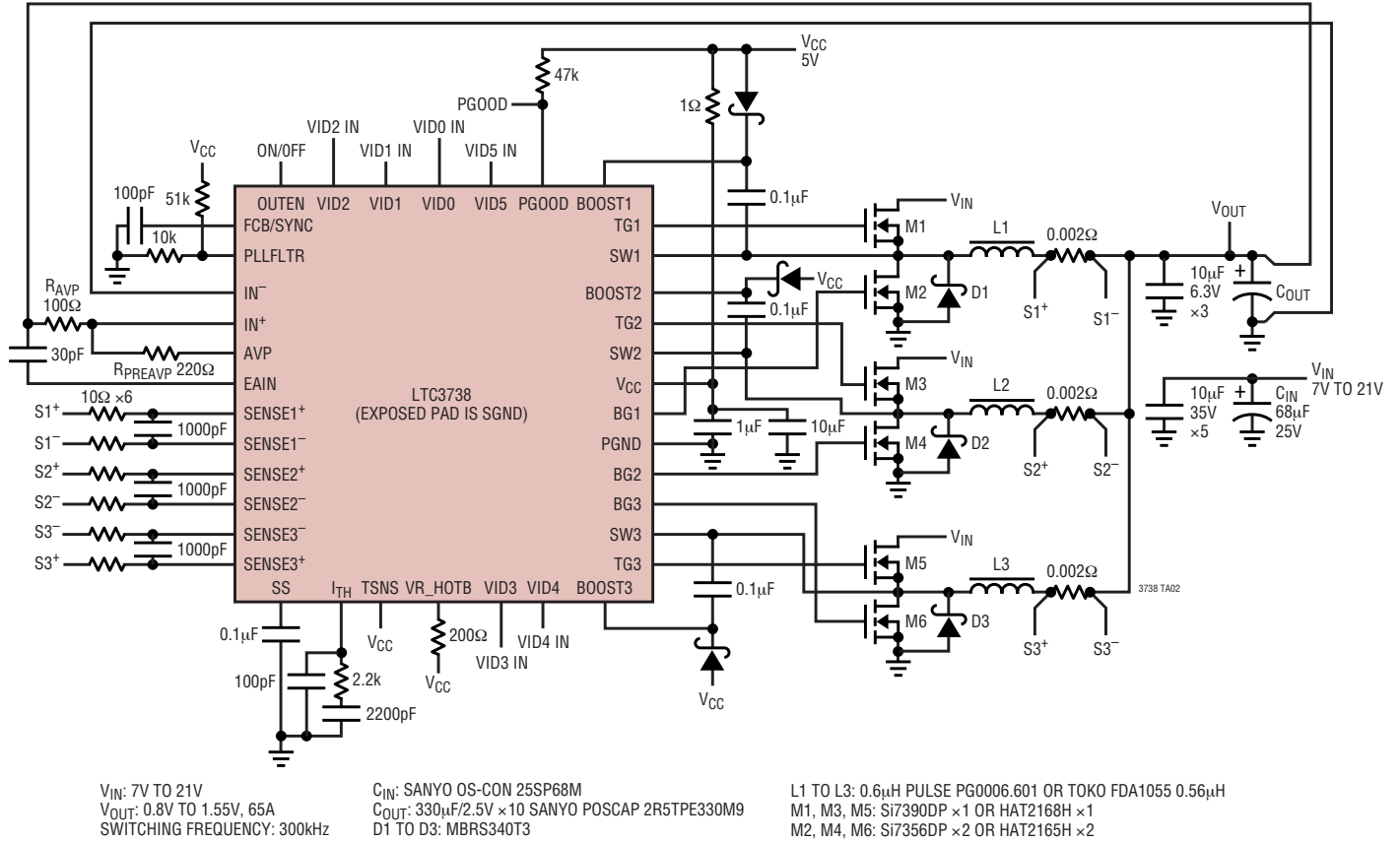
65A Power Supply for VRM10
