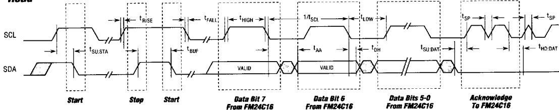
Figure 3. Bus Timing
