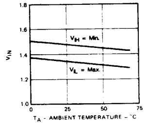
Typical VIN Limits Versus Ambient Temperature
