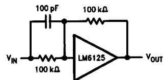
FIGURE 1. LM6125 with Overvoltage Protection
