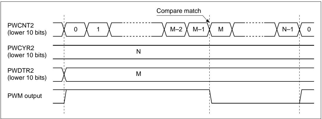
Figure 19-6 Duty Register Compare Match (OPS = 0 in PWPR2)
