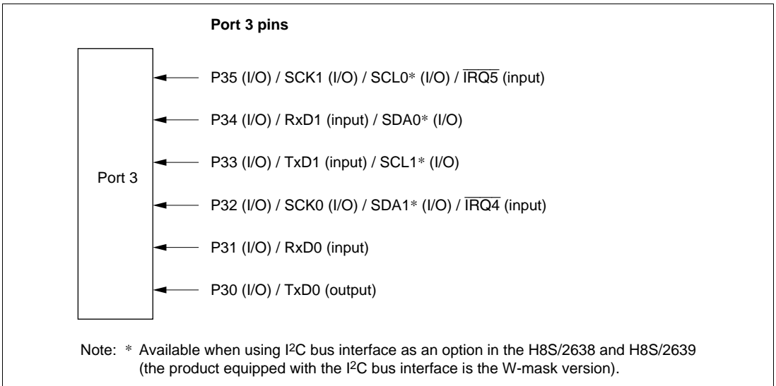
Figure 9-2 Port 3 Pin Functions
