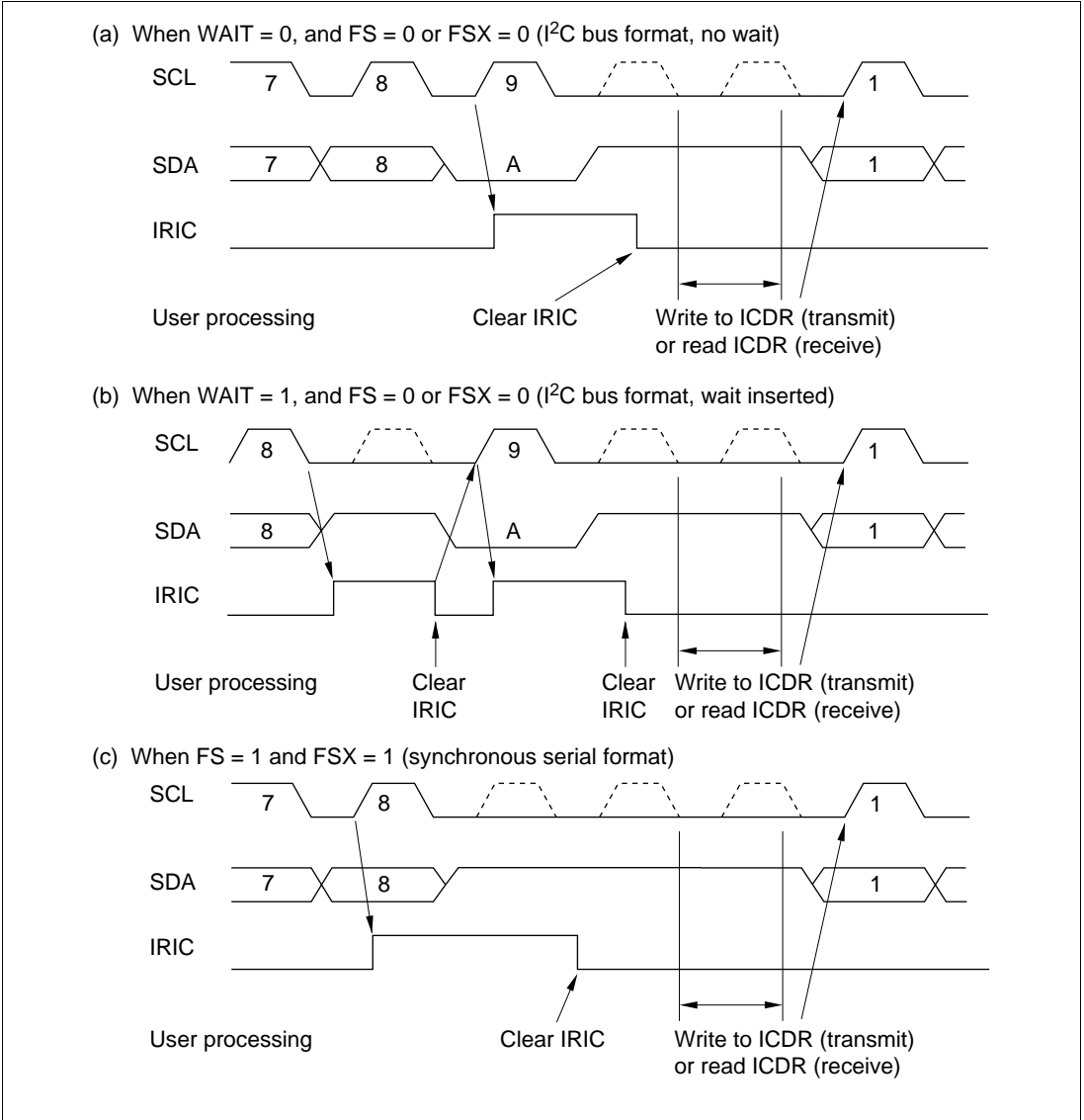
Figure 15-17 IRIC Setting Timing and SCL Control
