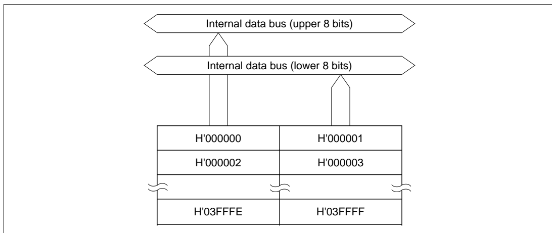
Figure 21B-1 Block Diagram of ROM (256 kbytes)
