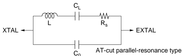
Figure 22A-3 Crystal Resonator Equivalent Circuit
