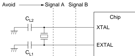
Figure 22A-4 Example of Incorrect Board Design
