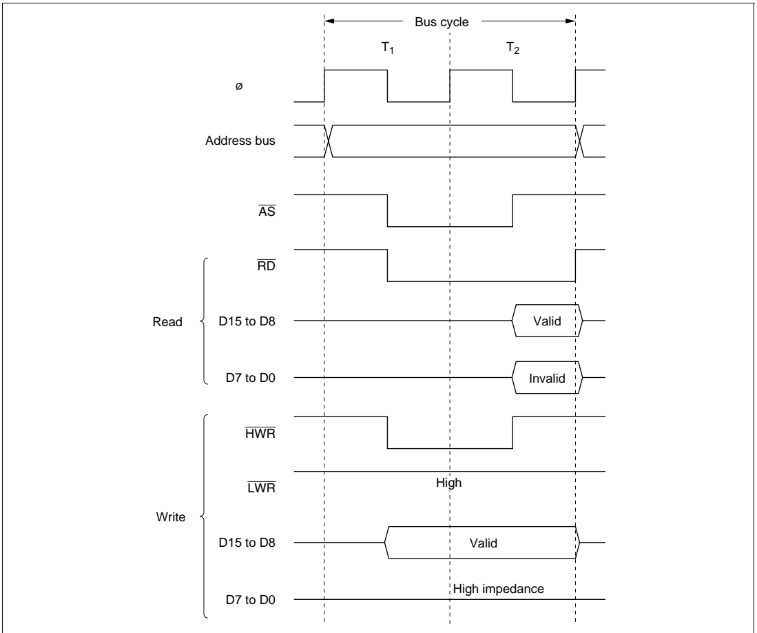
Figure 7-5 Bus Timing for 8-Bit 2-State Access Space
