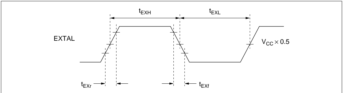
Figure 22A-7 External Clock Input Timing
