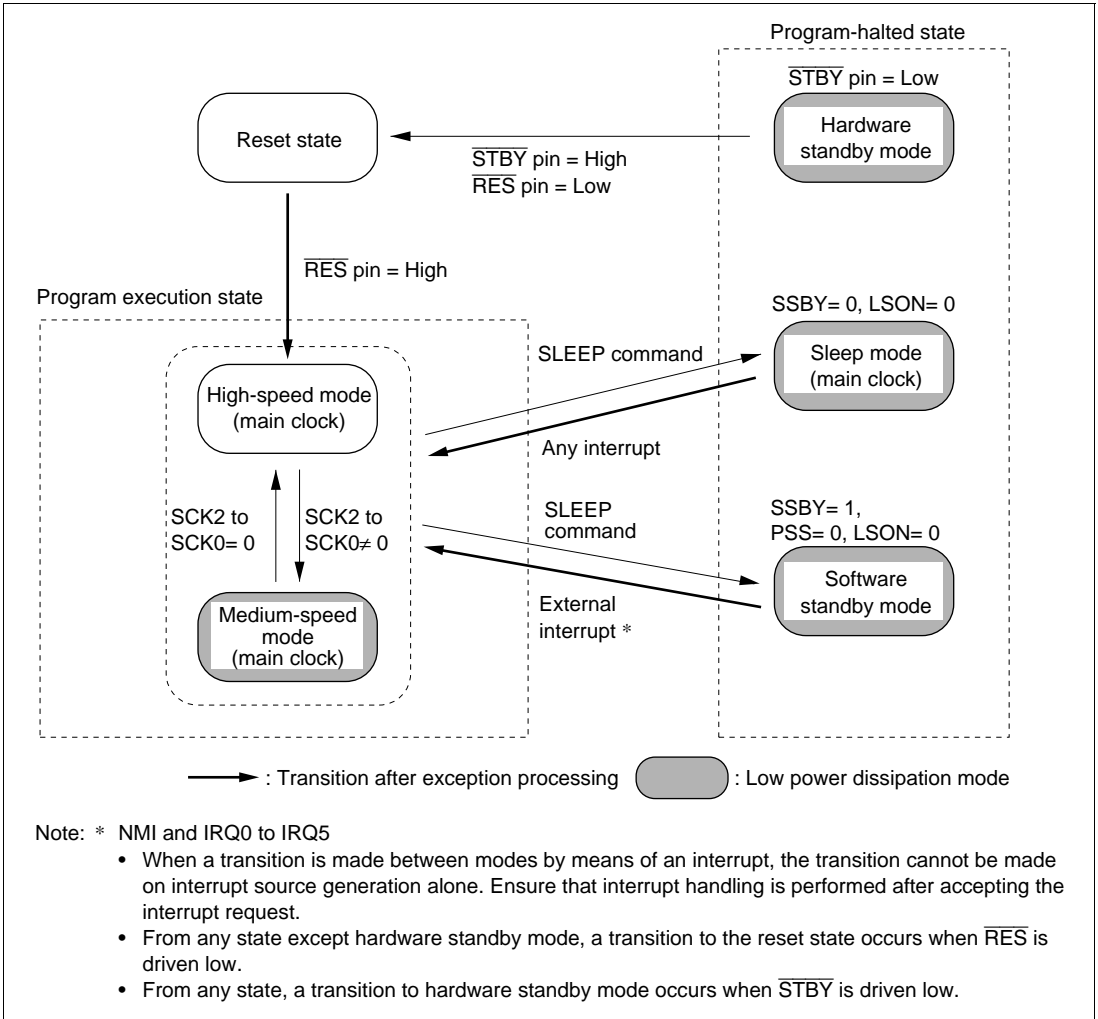
Figure 23A-1 Mode Transition Diagram
