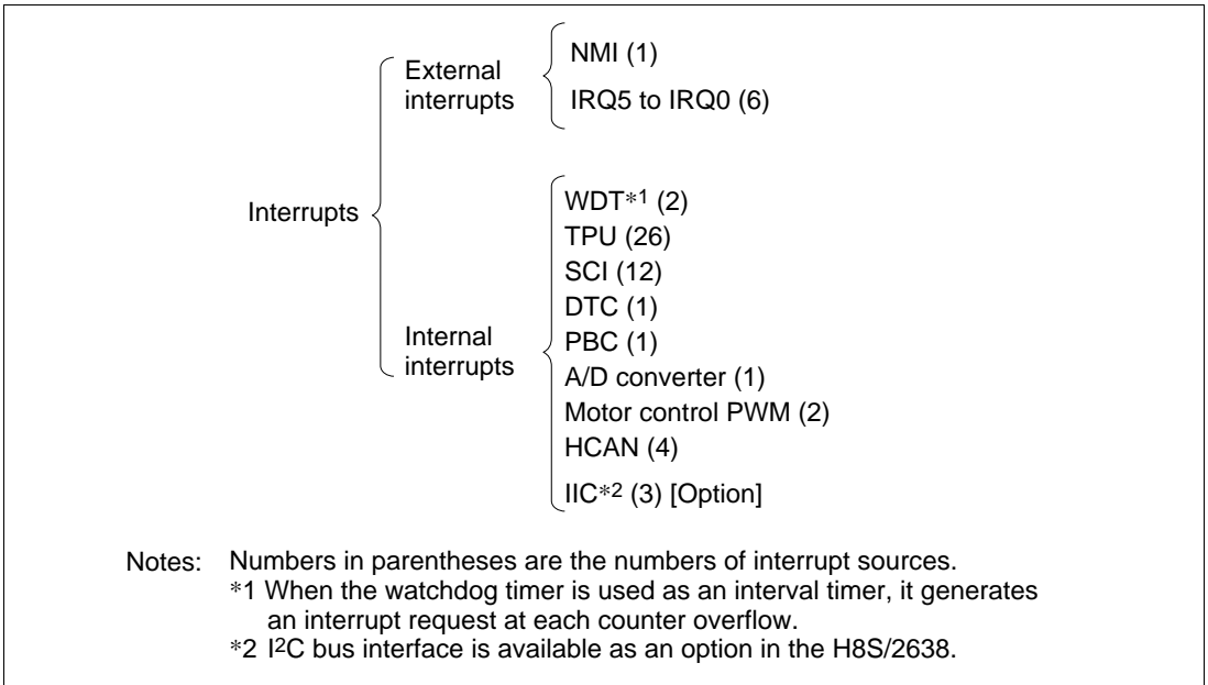
Figure 4-4 Interrupt Sources and Number of Interrupts
