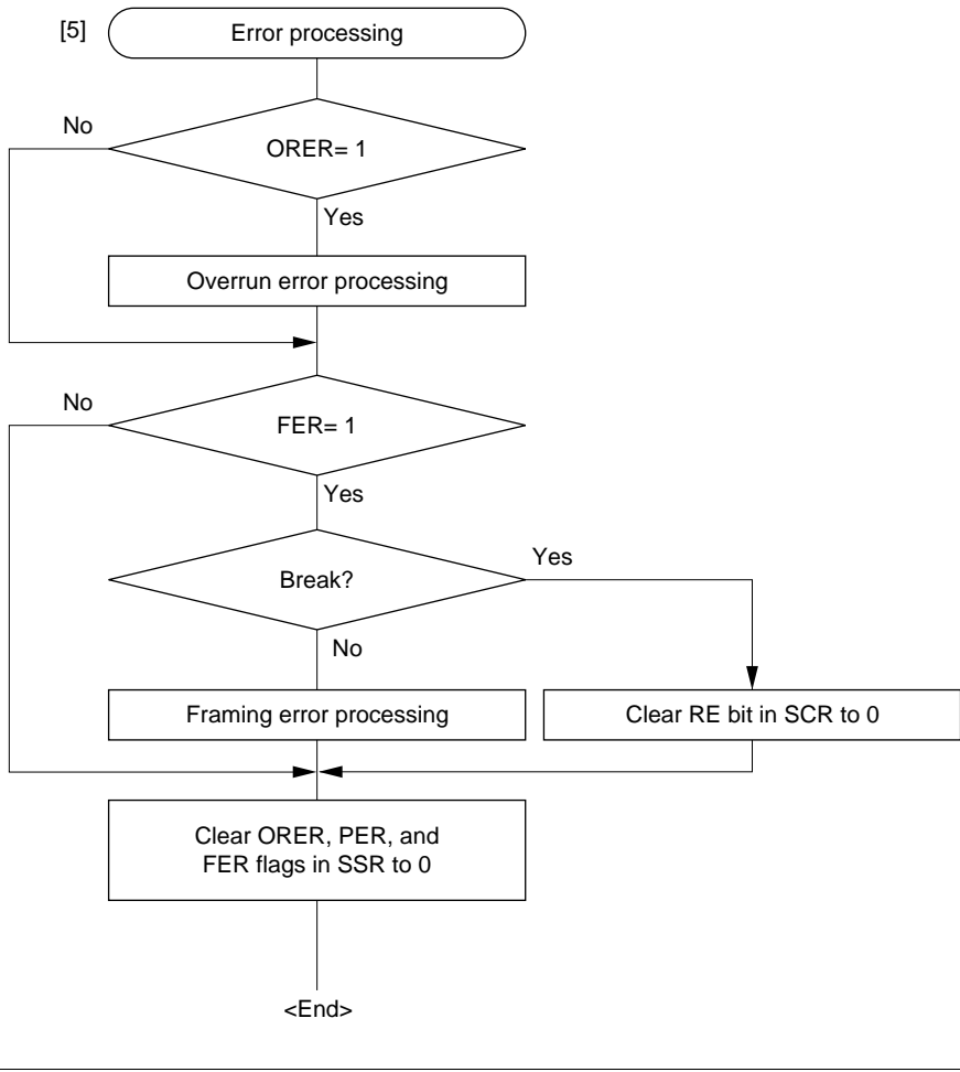
Figure 13-12 Sample Multiprocessor Serial Reception Flowchart (cont)
