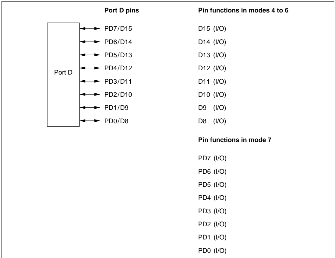
Figure 9-15 Port D Pin Functions
