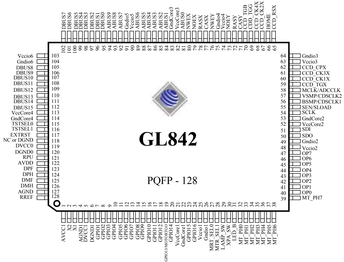
Figure 3.1 - Pinout Diagram
