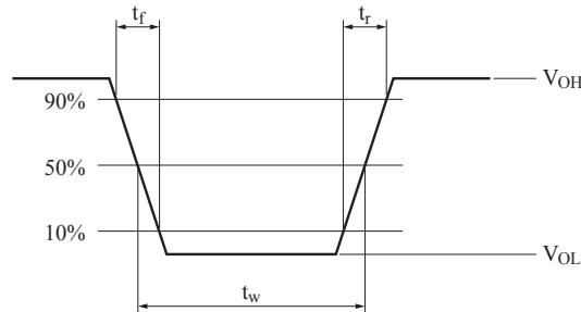
Fig.2 Output Waveform Specification(Receiver side)( C_L \leq 10pF )
