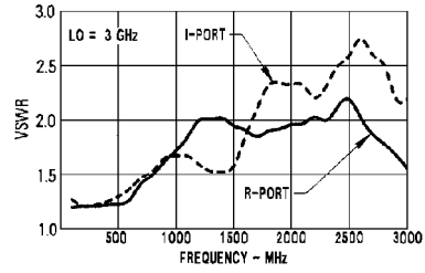
VSWR vs. Frequency
