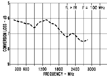
Conversion Loss vs. Frequency
