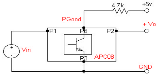
Figure 6. PGGood setup.
