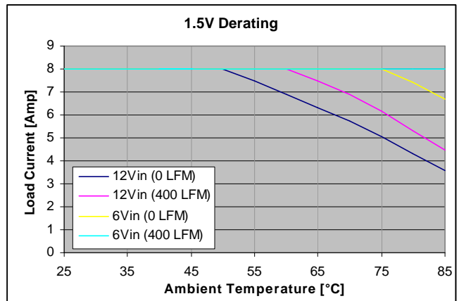
Figure 28. APC08M08 Thermal Derating Curve.
