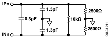
Figure 11. Receiver Simplified Equivalent Circuit When Driving Differentially
