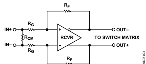
Figure 49. Input Receiver Equivalent Circuit
