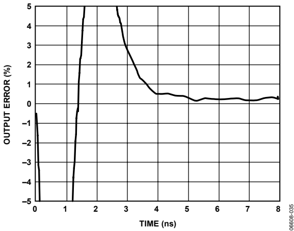
Figure 26. Settling Time, 1% Zoom
