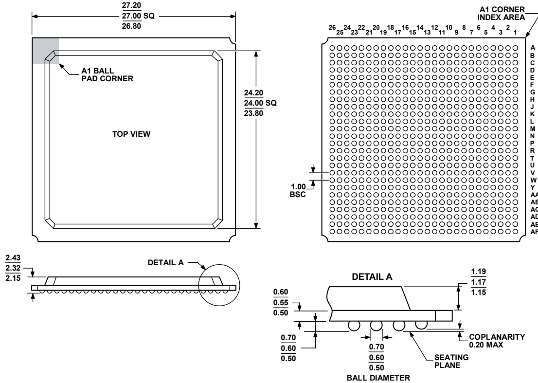
Figure 54. 676-Ball Plastic Ball Grid Array [PBGA] (B-676)
