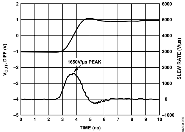
Figure 27. Large Signal Rising Edge Slew Rate
