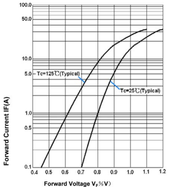
Fig.4 Forward Voltage
