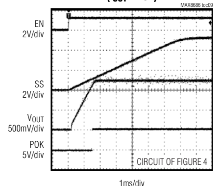
SOFT-START WITH EN CONTROL ( I_{OUT} = 10A )
