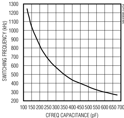
SWITCHING FREQUENCY vs. CFREQ CAPACITANCE
