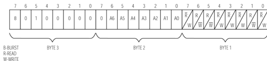
Figure 2. ADDRESS/COMMAND
