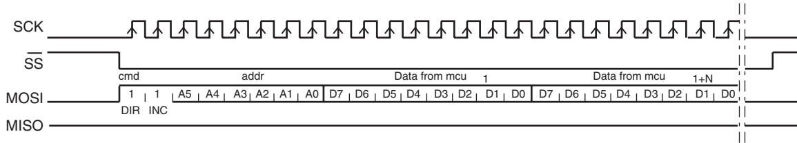
Figure 3-4. SPI Burst Write Sequence
