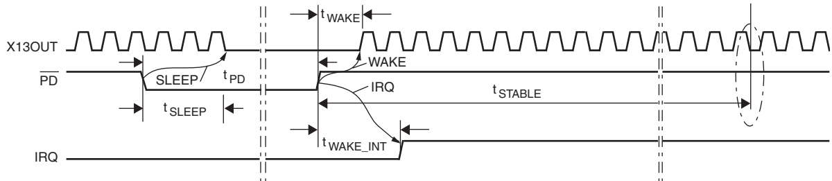
Figure 11-2. Sleep/Wake Timing
