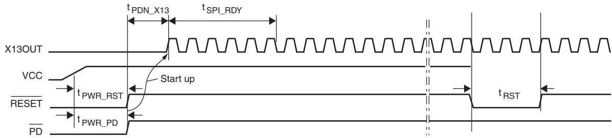
Figure 11-1. Power On Reset/Reset Timing
