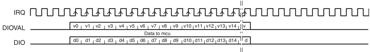
Figure 3-5. DIO Receive Sequence
