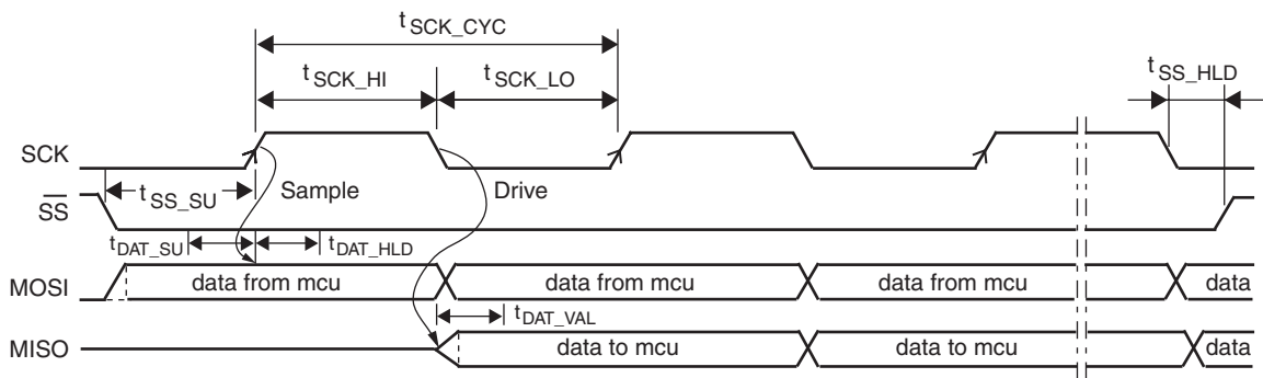
Figure 8-1. SPI Timing Diagram
