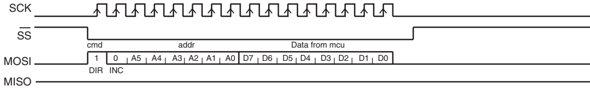
Figure 3-3. SPI Single Write Sequence
