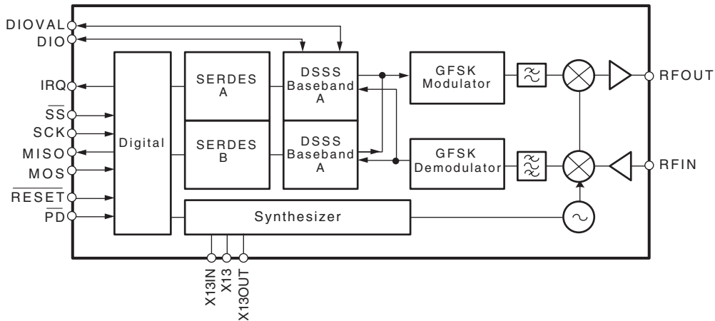
Figure 0-1. Simplified Block Diagram
