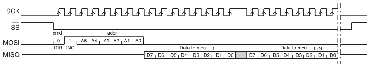
Figure 3-2. SPI Burst Read Sequence
