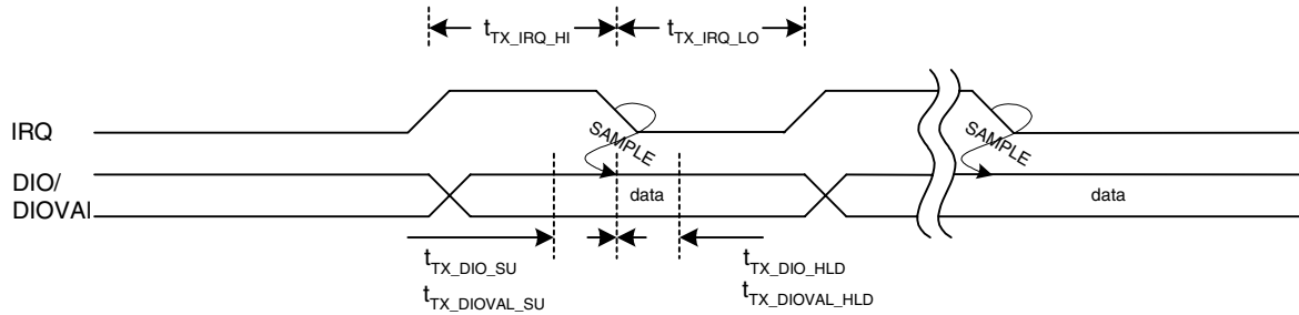
Figure 9-2. DIO Transmit Timing Diagram
