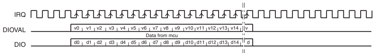
Figure 3-6. DIO Transmit Sequence
