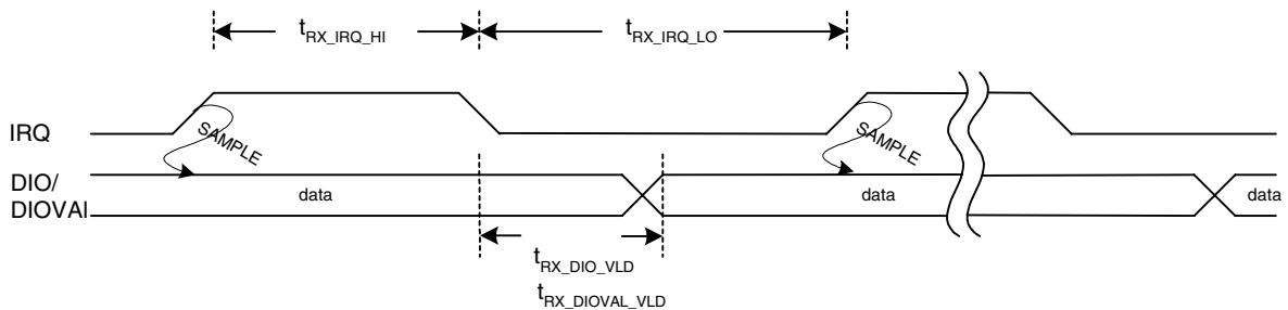
Figure 9-1. DIO Receive Timing Diagram
