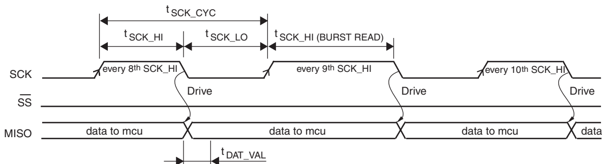
Figure 8-2. SPI Burst Read Every 9th SCK HI Stretch Timing Diagram
