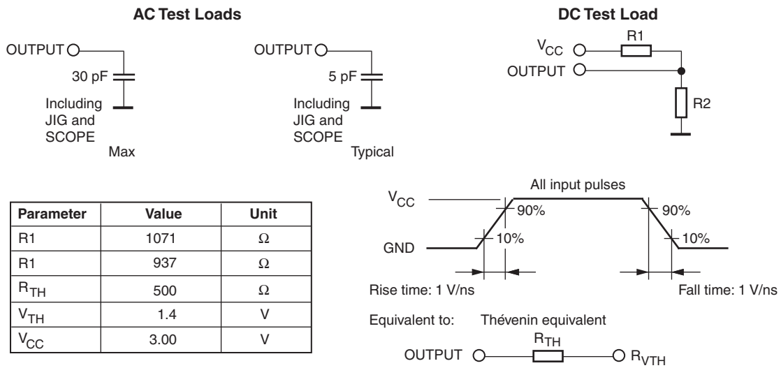
Figure 12-1. AC Test Loads and Waveforms for Digital Pins
