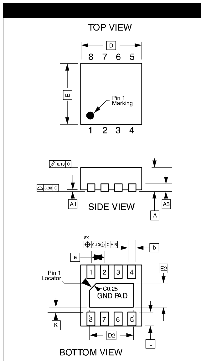
Dimensions for 8-Lead, 0.5mm pitch uDFN package
