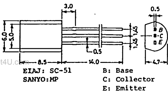
Case Outline—[2006A] unit:mm
