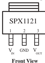
SOT-223 Package (M3)
