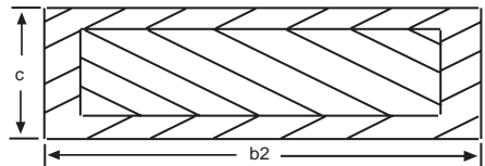
Section C-C
