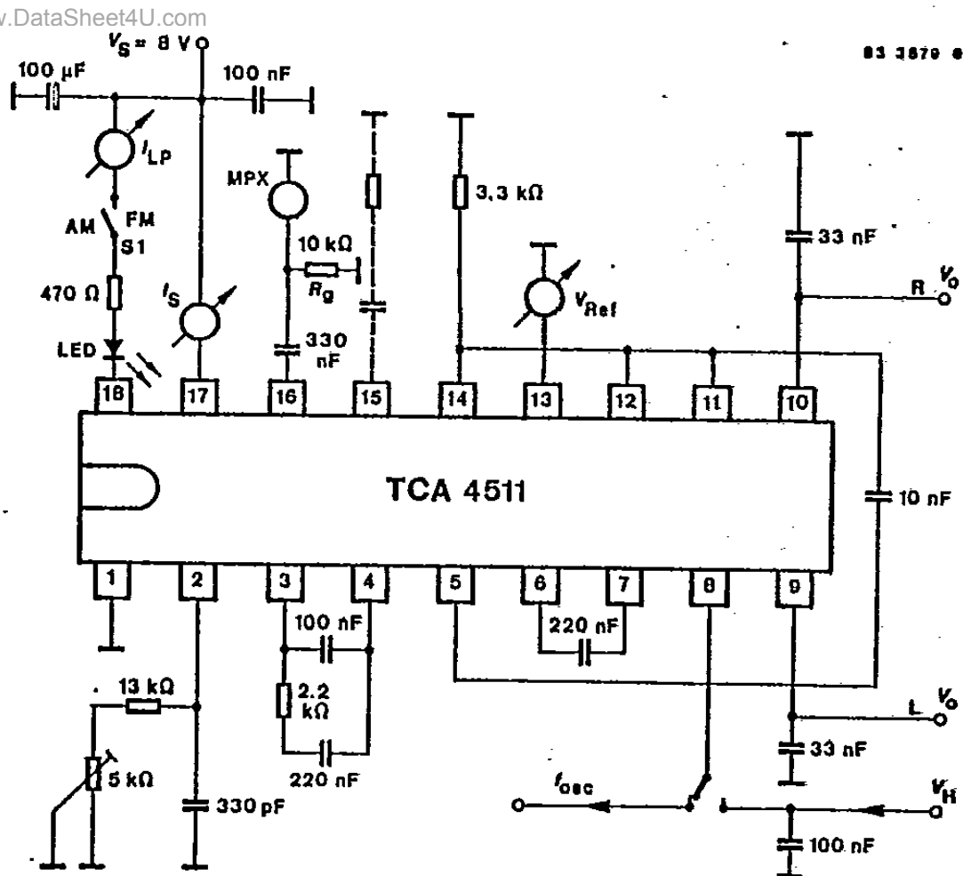
Fig. 2 Test circuit
