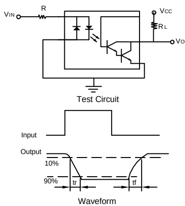
Switching Time Test Circuit
