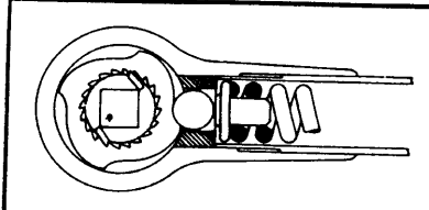
Working principle of Torqueleader Torque Safe
