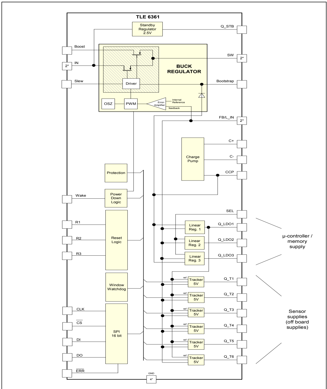
Figure 2 Block Diagram
