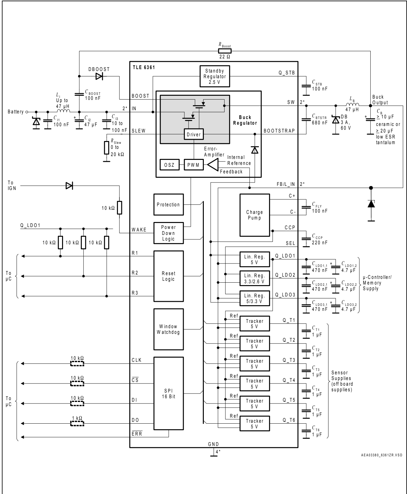
Figure 14 Application Diagram
