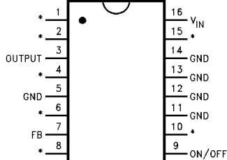
Top View LM2575N-XX or LM2575HVN-XX See NS Package Number N16A
