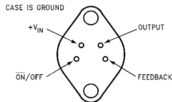
Bottom View LM1575K-XX or LM1575HVK-XX/883 See NS Package Number K04A
