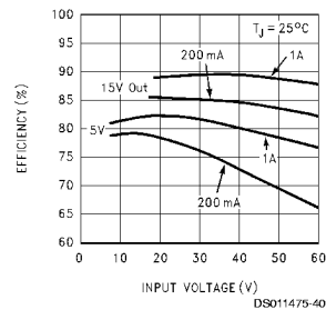
Efficiency
