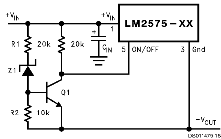
FIGURE 13. Undervoltage Lockout for Buck-Boost Circuit
