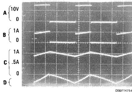
Switching Waveforms
