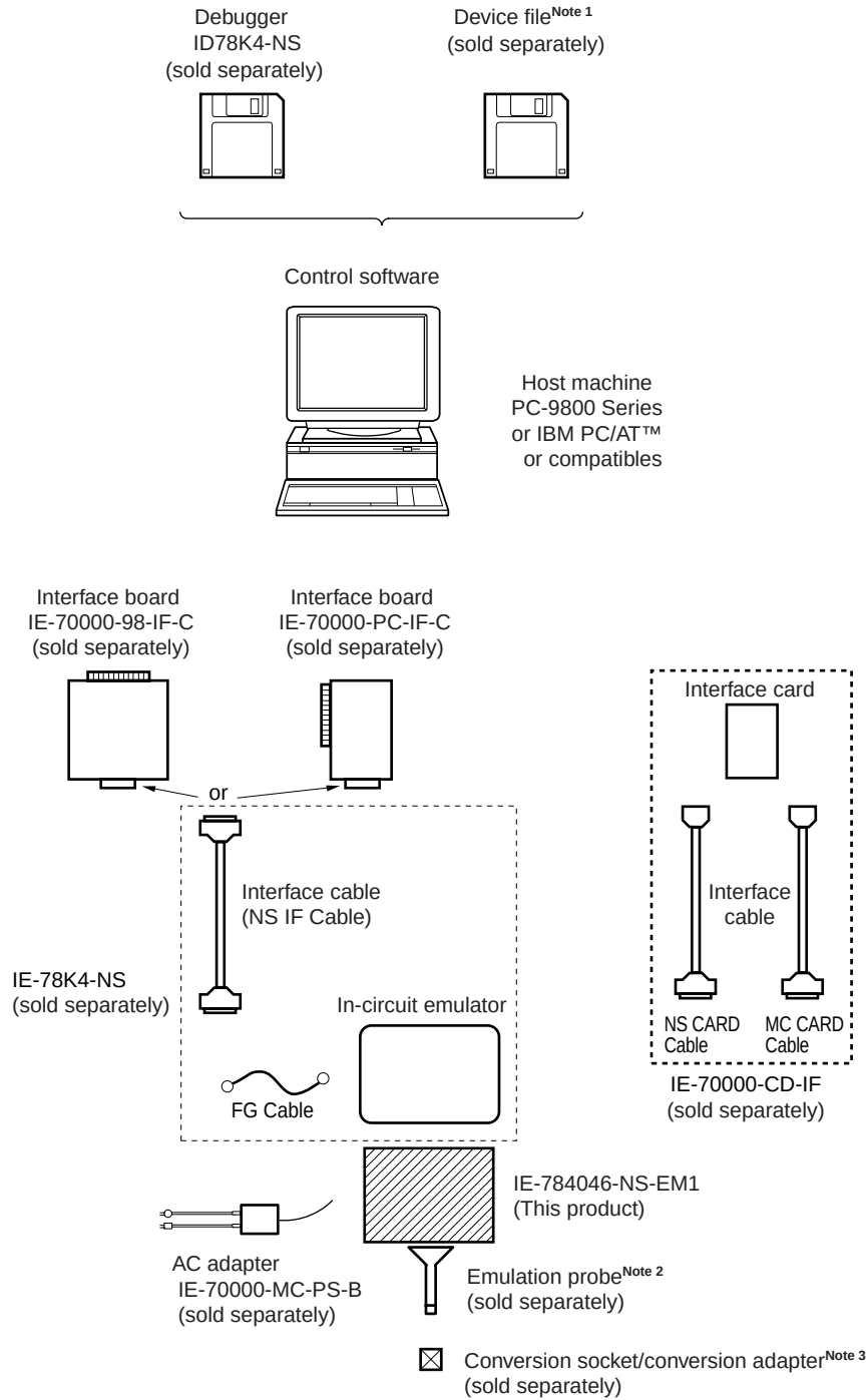
Figure 1-1. System Configuration
