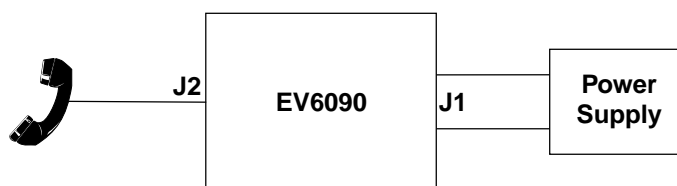
Figure 4: POTS Set-Up
