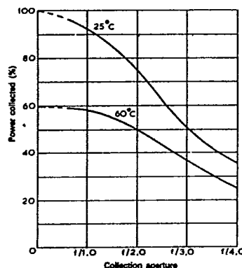
Fig 1 POWER VERSUS COLLECTION APERTURE
