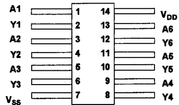
14-Lead Flatpack Top View
