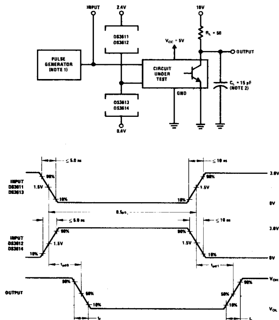
FIGURE 6. Switching Times of Complete Drivers
