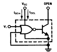
FIGURE 5. I_{CCH} , I_{CCL} for OR, NOR Circuits
