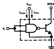
FIGURE 4. I_{CCH} , I_{CCL} for AND, NAND Circuits
