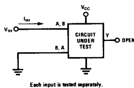
FIGURE 2. I_{IH} , I_{IL}
