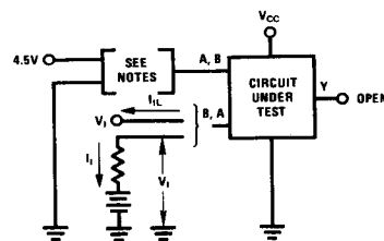
FIGURE 1. V_{IH} , V_{IL} , V_{OH} , V_{OL}
